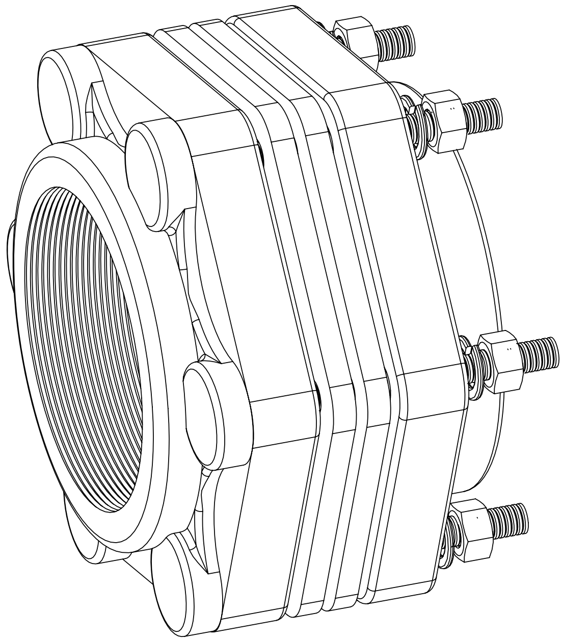
PART# 20089-1 EXPLODED VIEW
