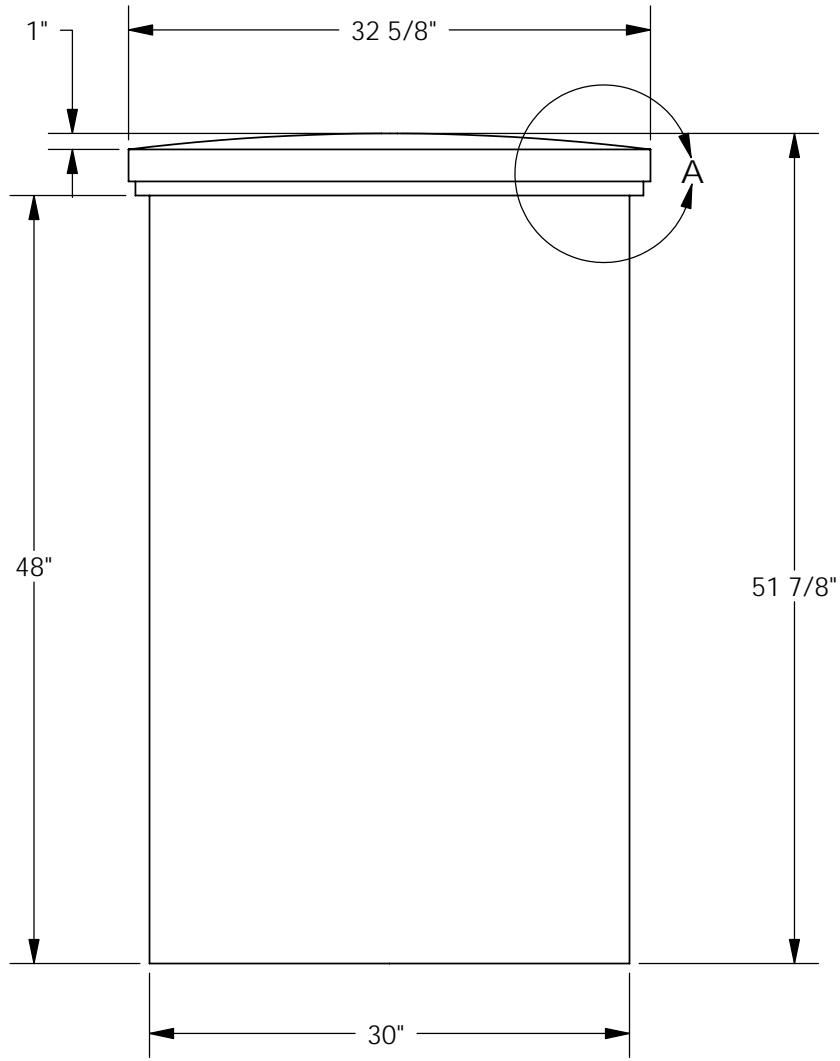
FRONT VIEW
