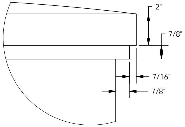
DETAIL A
